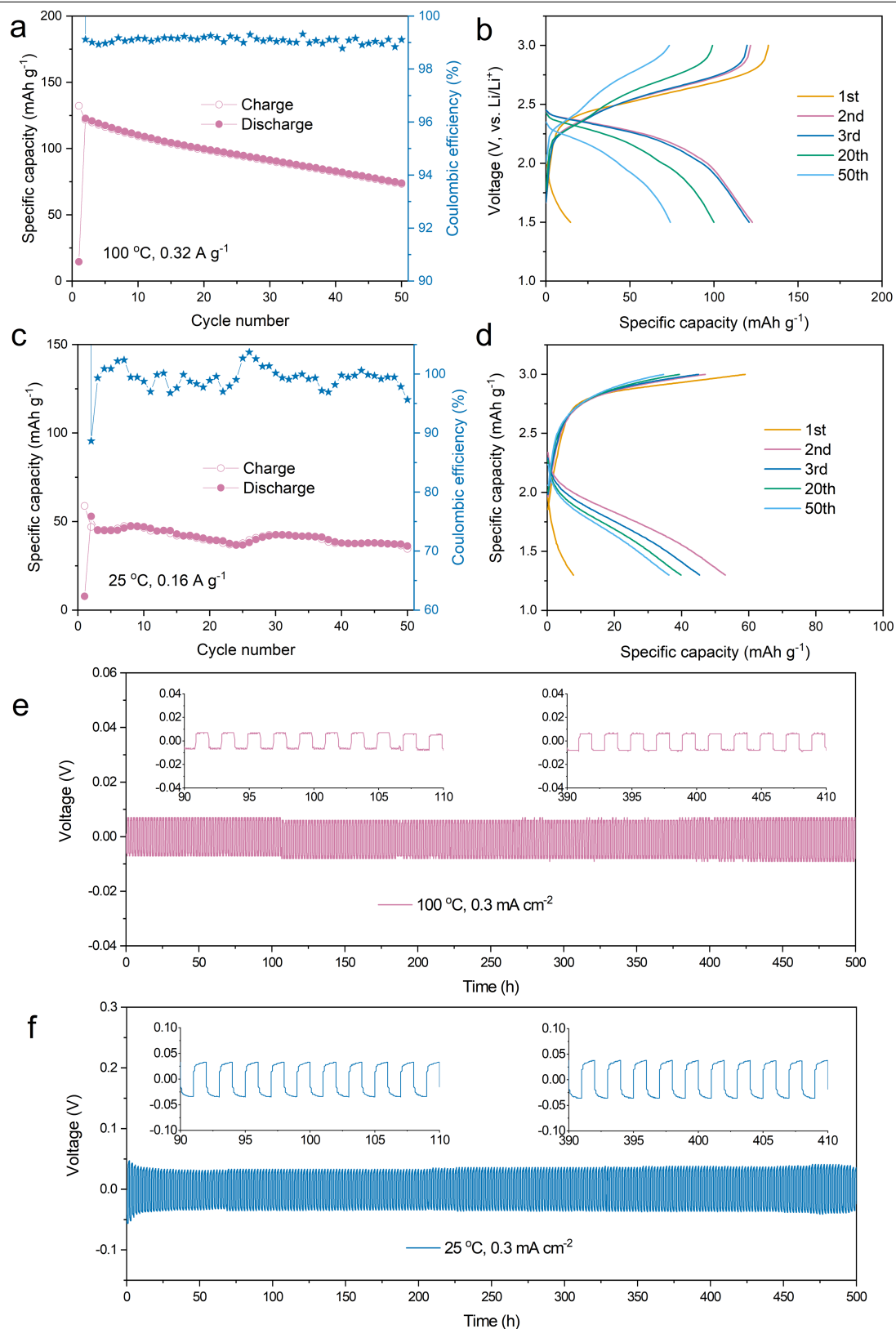
Extended Data Fig. 5 | Electrochemical performance data of solid state cell components. The cycling stability and capacity of a LPS/VGCF cathode at 100\text{ }^{\circ}\text{C} (a) and 25\text{ }^{\circ}\text{C} (c). The corresponding voltage profiles at 100\text{ }^{\circ}\text{C} (b) and at 25\text{ }^{\circ}\text{C} (d). Capacity contribution of LPS is very limited and the cycling stability
