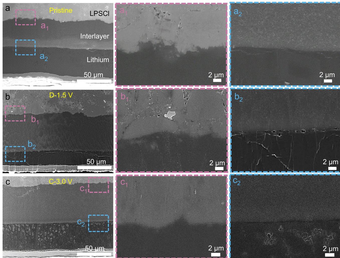
Extended Data Fig. 7 | Morphological study of the Li-SP-LPSCI interface during cycling in full cells. The cross-sectional SEM of Li/SP/LPSCI interface at different states: pristine (a), fully discharged to 1.5 V (b) and fully charged back to 3.0 V (c). It should be noted that all of the anode interfaces were cut from the full cells with the configuration of S_{9.3}I -LPS-VGCF/LPS/LPSCI/SP/Li with a high mass loading of S_{9.3}I 4.2 \text{ mg cm}^{-2} running at 100^\circ\text{C} and at a current density of 0.32 \text{ A g}^{-1} . At the pristine state (a), both the Li/SP interface and SP/LPSCI SSE
