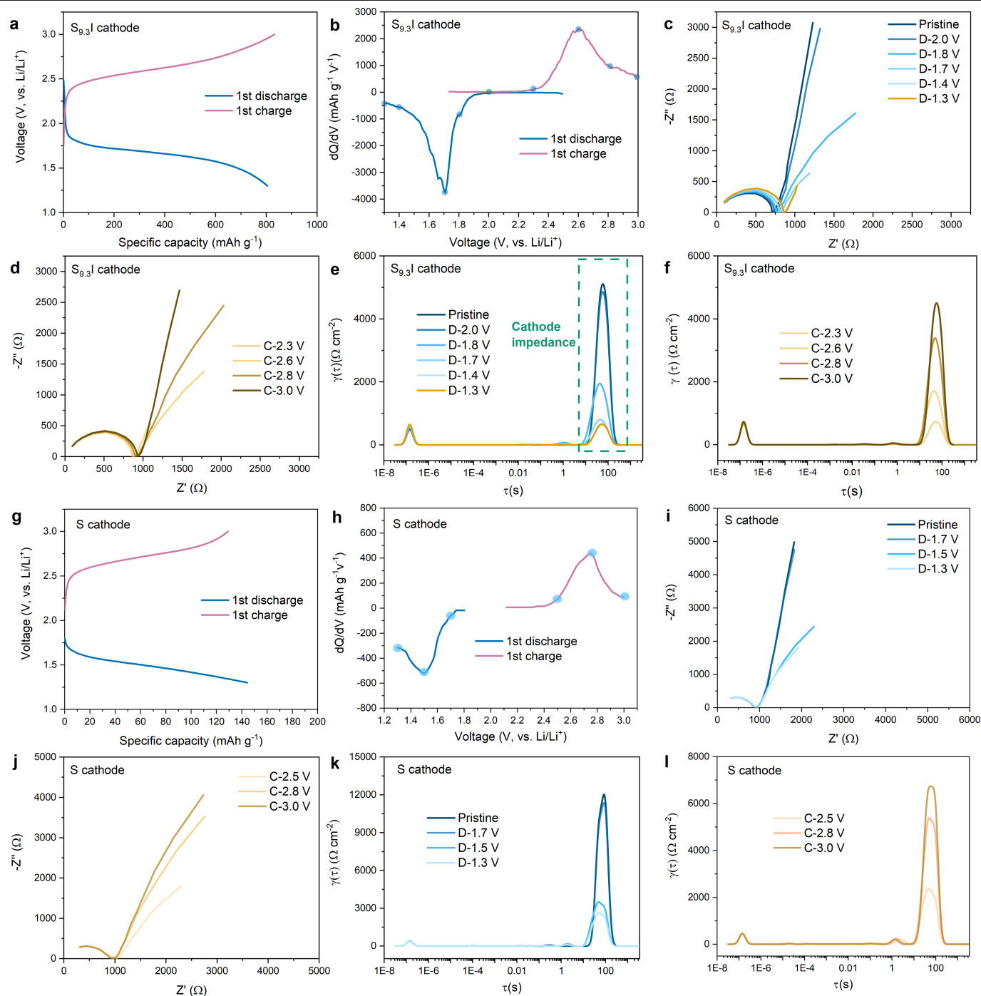
Extended Data Fig. 8 | EIS study of Li-S 9.3 I and Li-S full cell at 25 °C during initial cycles. (a) The initial discharge/charge curves of a Li-S 9.3 I cell, and the corresponding dQ/dV curves (b) derive from (a). (c) The EIS of the Li-S 9.3 I cell at different states of discharge. (d) The EIS of the Li-S 9.3 I cell at different states of charge. The DRT analysis of EIS at different states of discharge (e) related to (c), and states of charge (f) related to (d). (g) The initial discharge/charge curves of
