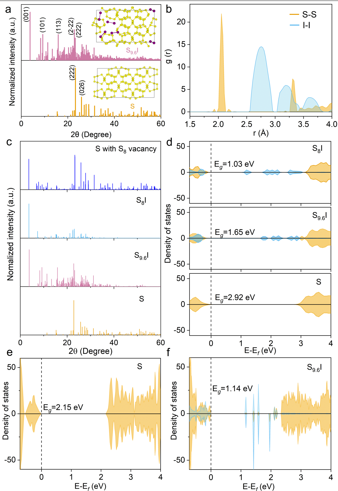
Extended Data Fig. 2 | Computed Crystal and electronic structure of S-I compounds. (a) Computed XRD patterns of elemental S and predicted S_{9.6}I structure. (b) Computed PDF of S_{9.6}I . We attribute any minor discrepancies to the fact that the DFT relaxations are carried out at 0 K, while the experimental
