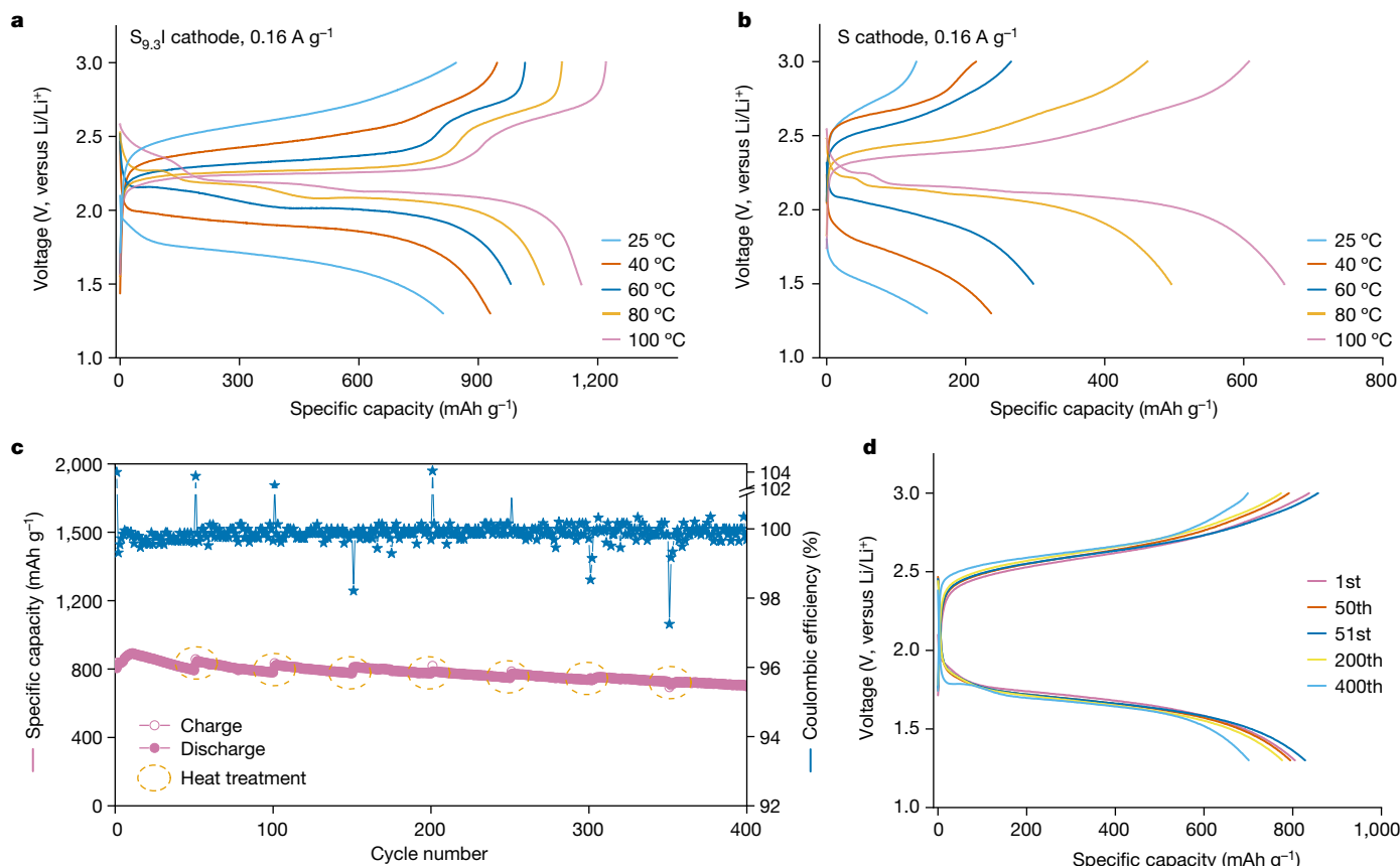
Fig. 2 | The electrochemical performance of S_{9.3}I and elemental S cathodes in solid-state Li-S cells. a, b , Discharge/charge profiles of S_{9.3}I cathode (a) and elemental S cathode (b) at 0.16 \text{ A g}^{-1} from 25^\circ\text{C} to 100^\circ\text{C} . c , Long-term cycling
