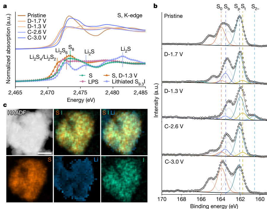
Fig. 3 | The working mechanism of S 9.3 I cathode in Li-S 9.3 I cell at 25 °C. a , SK-edge XAS spectra of S 9.3 I cathode during the initial cycle. b , S 2p high resolution XPS of S 9.3 I cathode during the initial cycle. c , Cryo-TEM HAADF (high-angle
