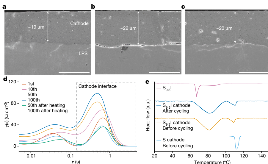
Fig. 4 | Repair of the S 9.3 I cathode/LPS solid electrolyte interface in Li-S 9.3 I cells by remelting. a–c , Cross-sectional SEM images of S 9.3 I cathode/LPS interface at 25 °C: before cycling (a), after 50 cycles (b) and after reheating at 100 °C after 50 cycles (c). d , DRT analysis of EIS data of the Li-S 9.3 I full cell after
