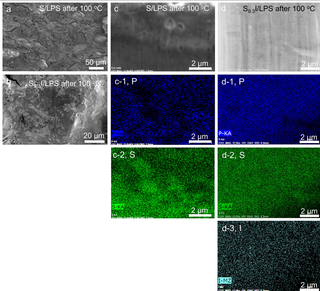
Extended Data Fig. 4 | SEM and elemental mapping of S and S_{9.3}I mixed with LPS after heating at 100 °C. The SEM image of S/LPS mixture (a) and S_{9.3}I /LPS mixture (b) after milling and heating at 100 °C. (c) The cross sectional cryo-FIB
