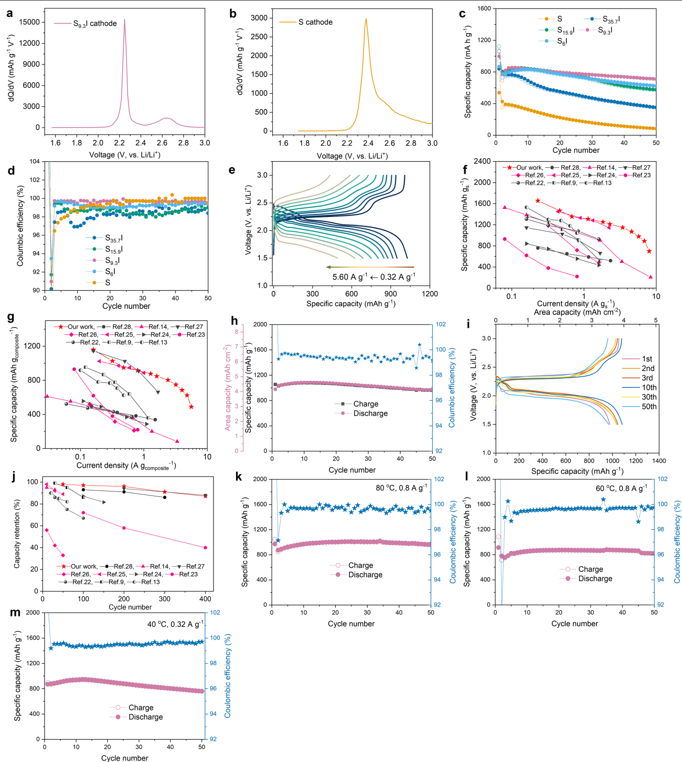
Extended Data Fig. 6 | The performance of sulfur iodide cathode at different conditions and their comparison with other SSLSBs. The dQ/dV curves during delithiation of \text{S}_{9.3}\text{I} (a) and S (b) cathode based on the charging curves at 100 °C from Figs. 2a and b. (c) The cycling stability of \text{S} , \text{S}_{35.7}\text{I} , \text{S}_{15.9}\text{I} , \text{S}_{9.3}\text{I} and \text{S}_6\text{I} cathode at 1.6 \text{A g}^{-1} and at 100 °C. (d) The corresponding cycling coulombic efficiency in (c). (e) Rate capability of \text{S}_{9.3}\text{I} cathode at 100 °C at current densities of 0.32, 0.48, 0.80, 1.28, 1.60, 2.40, 3.20, 4.00, 4.80 and 5.60 \text{A g}^{-1} . Rate performance comparison between Li- \text{S}_{9.3}\text{I} solid state batteries with other SSLSBs: based on the weight of (f) only S and (g) S composite, red-colored
